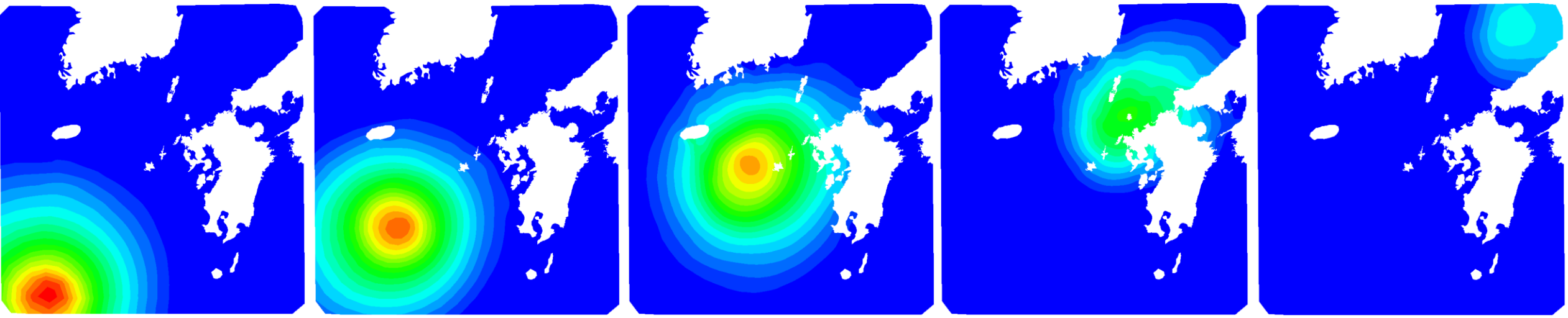
GPV(MSM)気圧
